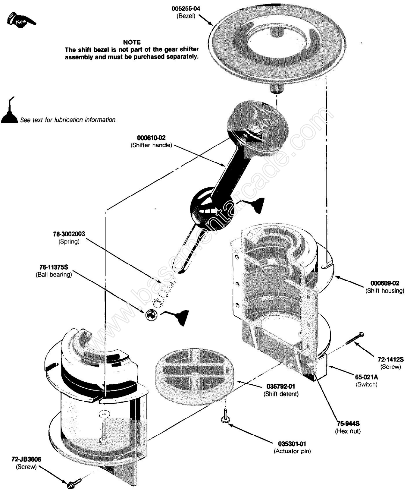
Figure 3-6 Gear-Shifter Control Assembly A000608-09 Y
