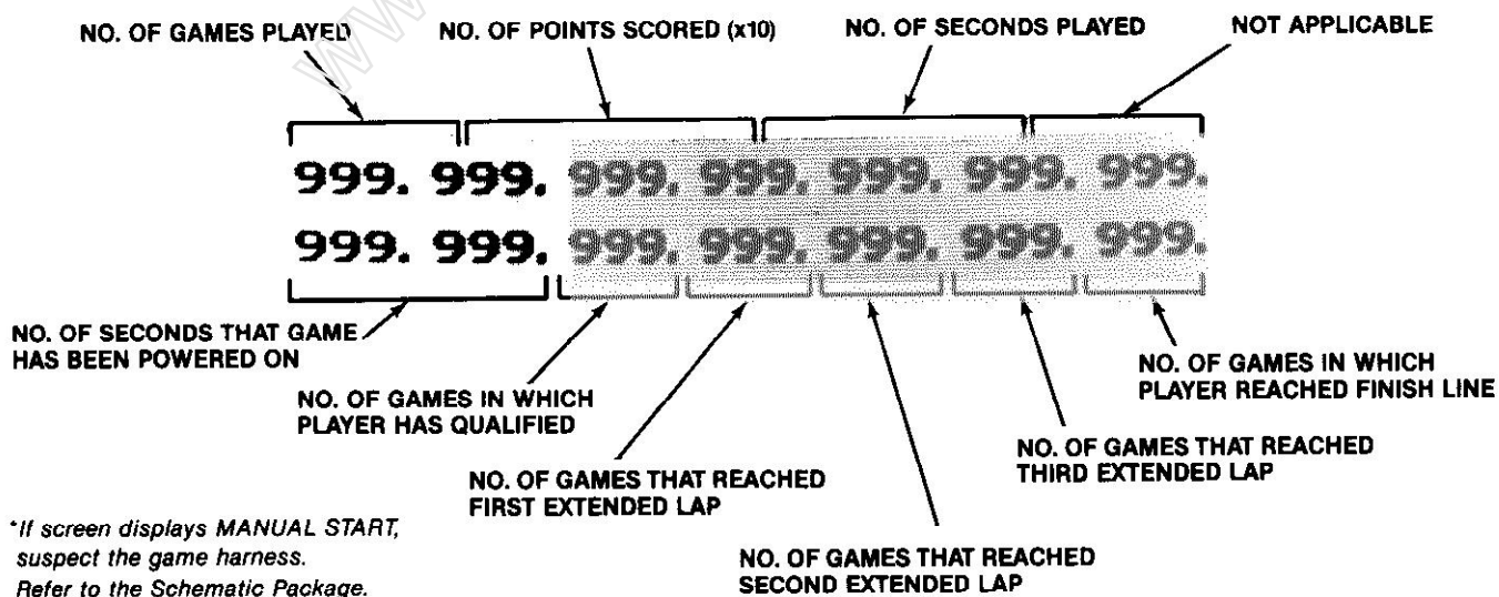
Figure 1-5 Self-Test Display
