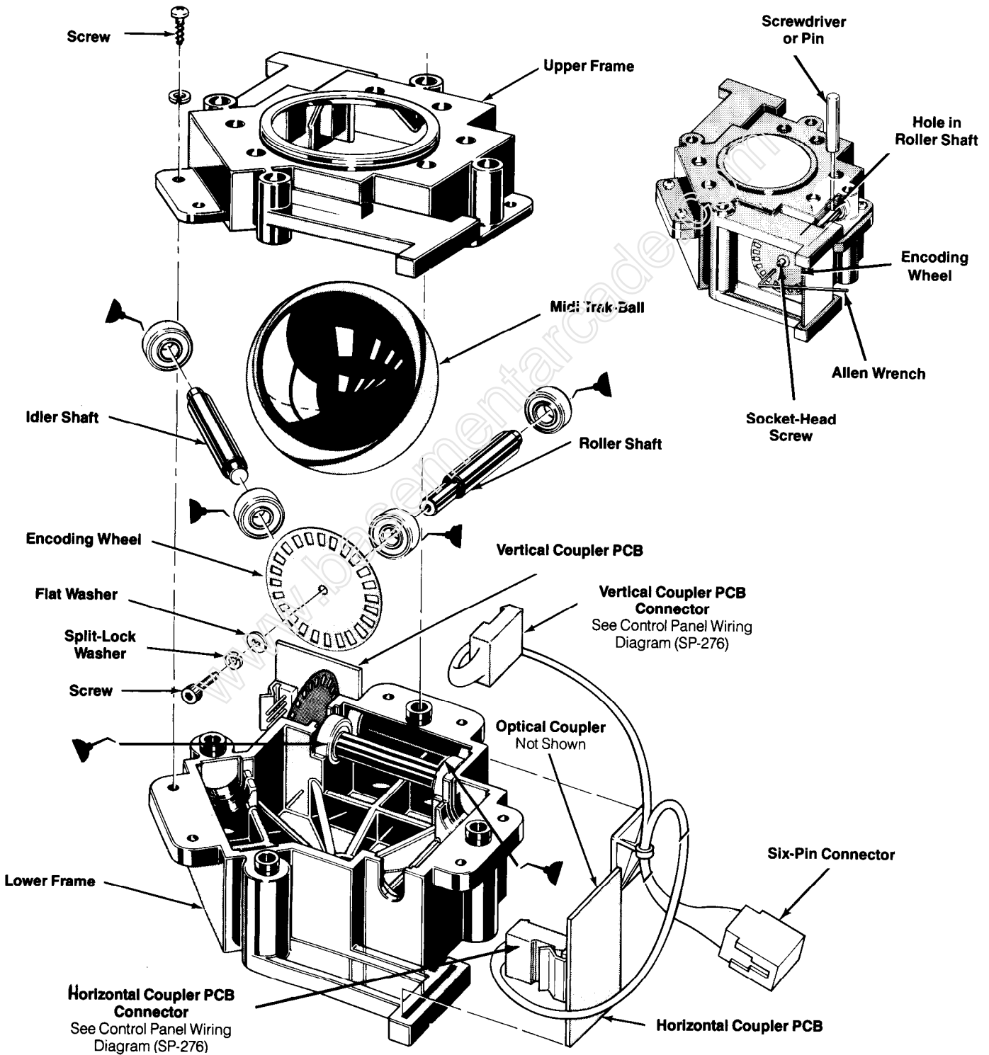
Figure 3-3 Midi Trak-Ball Disassembly and Lubrication
