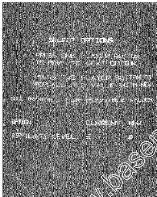
Figure 2-7 Select Options
